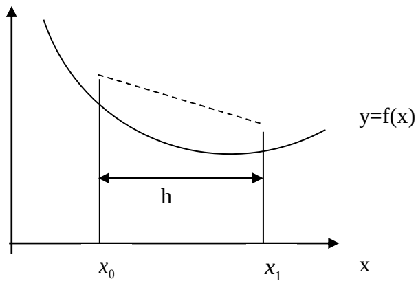
Gambar 4.4 Kaidah Trapesium
