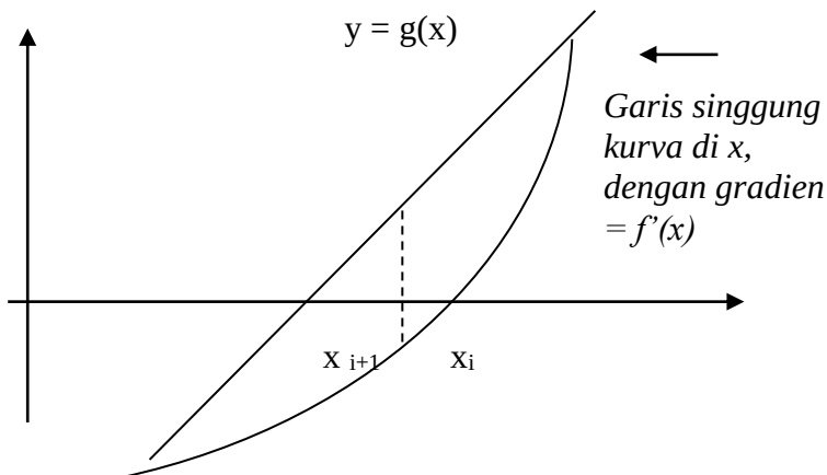
Gambar 2.3 Tafsiran geometri metode Newton-Raphson
